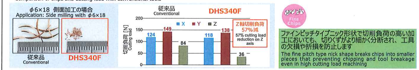
刃先形状 Cutting edge shape
